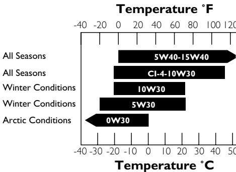
Fig.7.1. Recommended SAE Oil Viscosity Grades v.s. Ambient Temperatures
