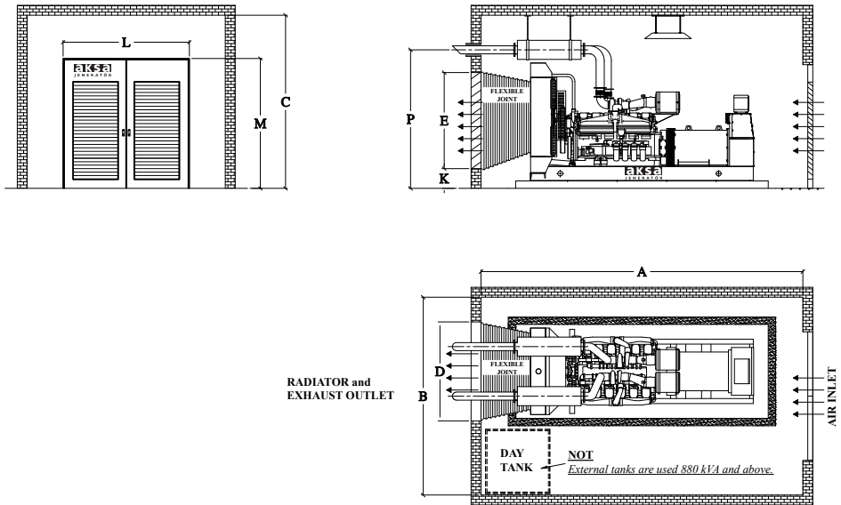
Figure 3.6. Generator set room
