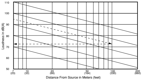
Figure 11.2. Decreases In Loudness As Distance Increases (Free Field)
